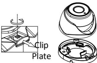
Figure 2-9 Remove the Clip Plate
