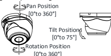
Figure 2-12 3-axis Adjustment
